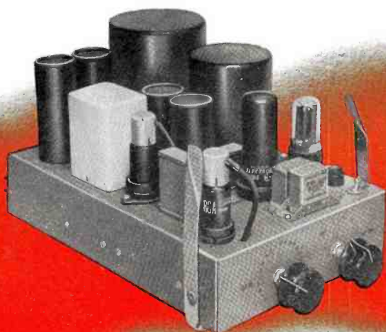
New Program Amplifier (type BA-13). The most versatile high-fidelity amplifier ever designed for broadcasting. Ideal as a program or line amplifier, bridging amplifier, isolator amplifier, cueing or monitoring amplifier. Improved layout for greater accessibility; "plug-in" electrolytics for ease in servicing. Output , 2 watts (approx.). Higher gain , 65 db for matching input; 28 db for bridging input. Lower noise level , -82 db (with max. gain). Lower distortion , less than 0.5 to 1% rms, depending on output level. Frequency response , \pm 1 db, 30 to 15,000 cps.
